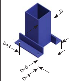
COLUMN BASE DETAIL FOR 3" COLUMNS
