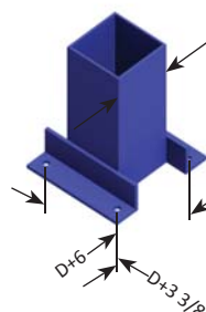
COLUMN BASE DETAIL FOR 4" & 5" COLUMNS
