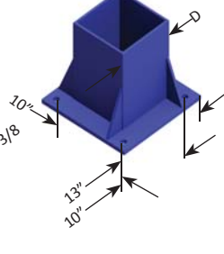
COLUMN BASE DETAIL FOR 6" & 7" COLUMNS
